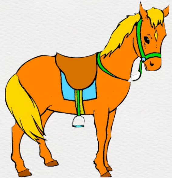
Horse
