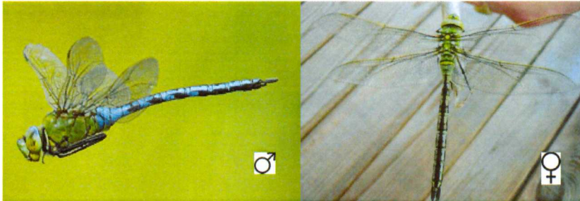
Anax imperator
